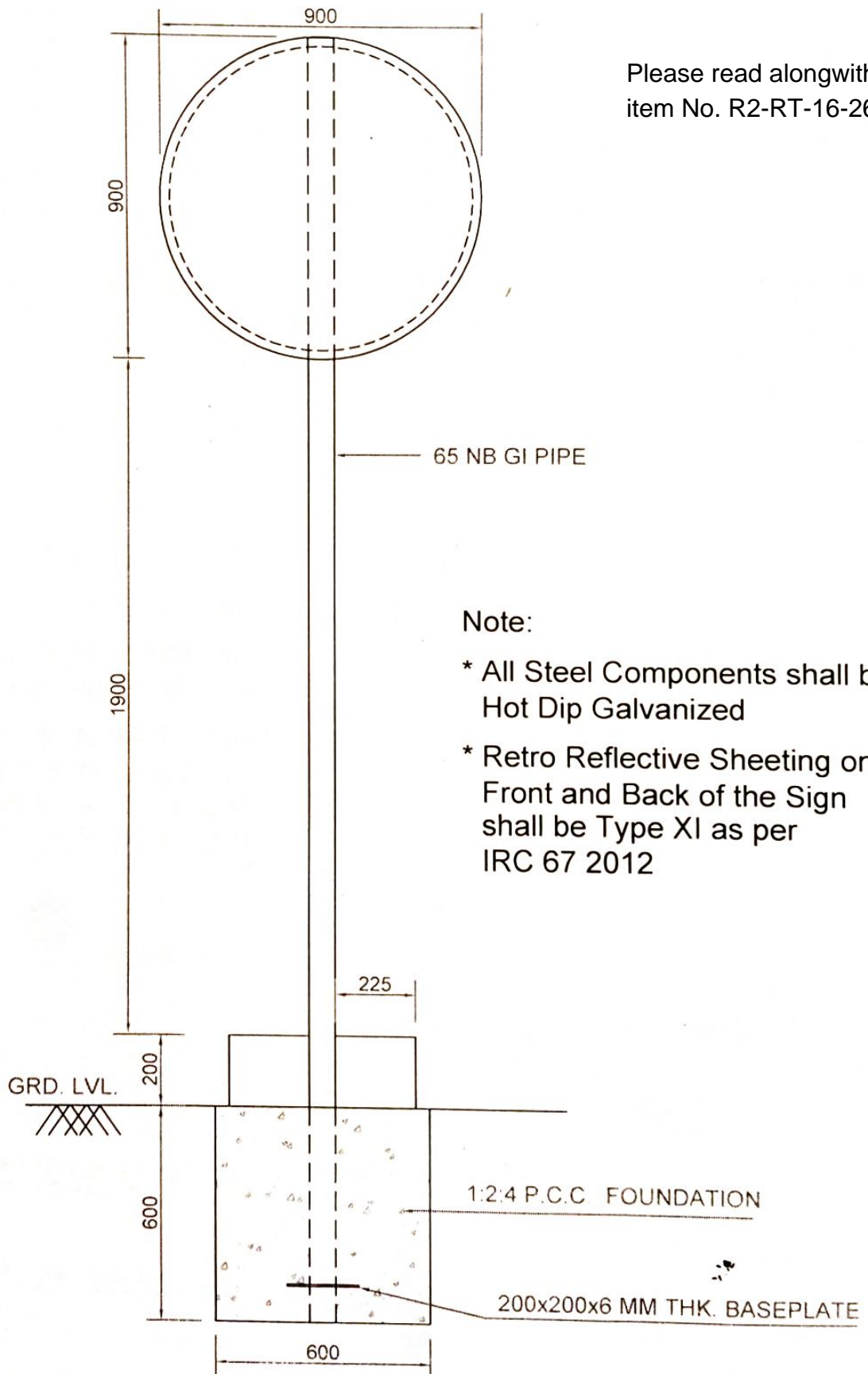
Mandatory Sign Drawing Refer Fig. M2
