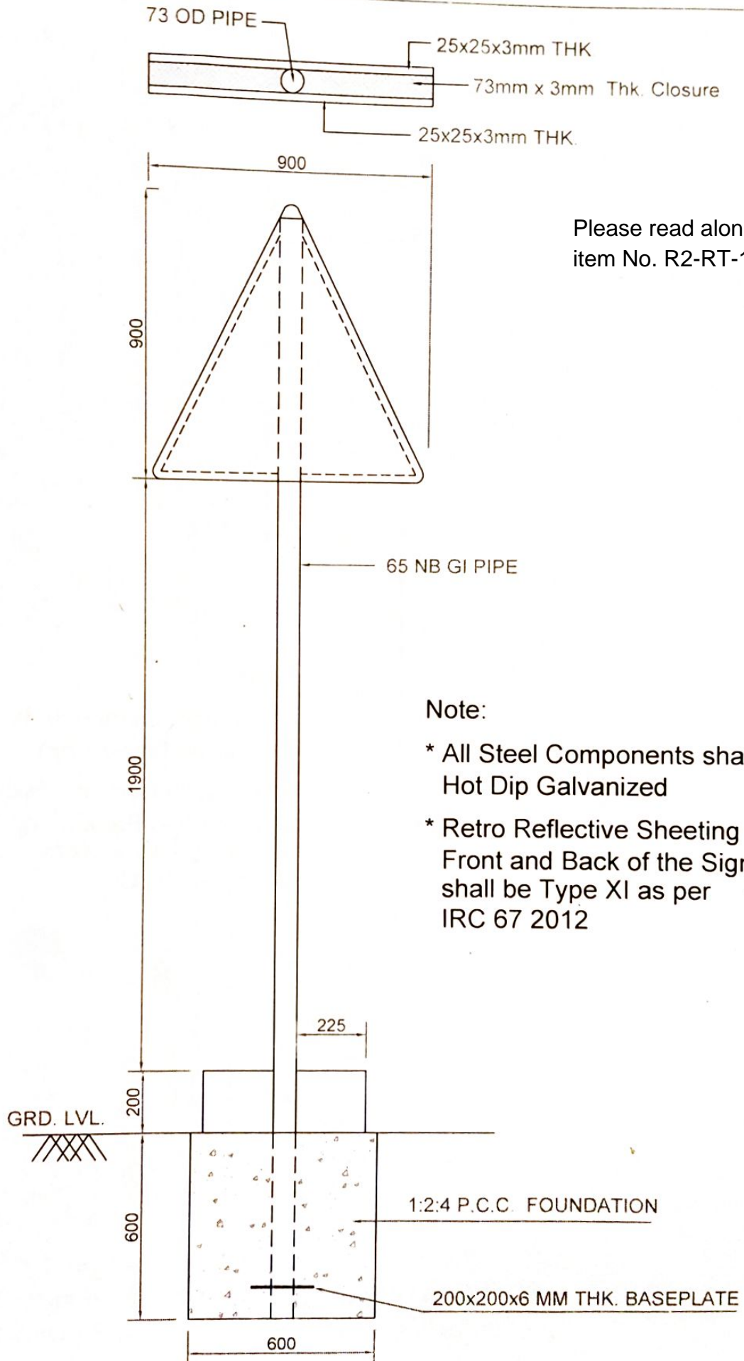
Cautionary Sign Drawing Refer Fig. C2
