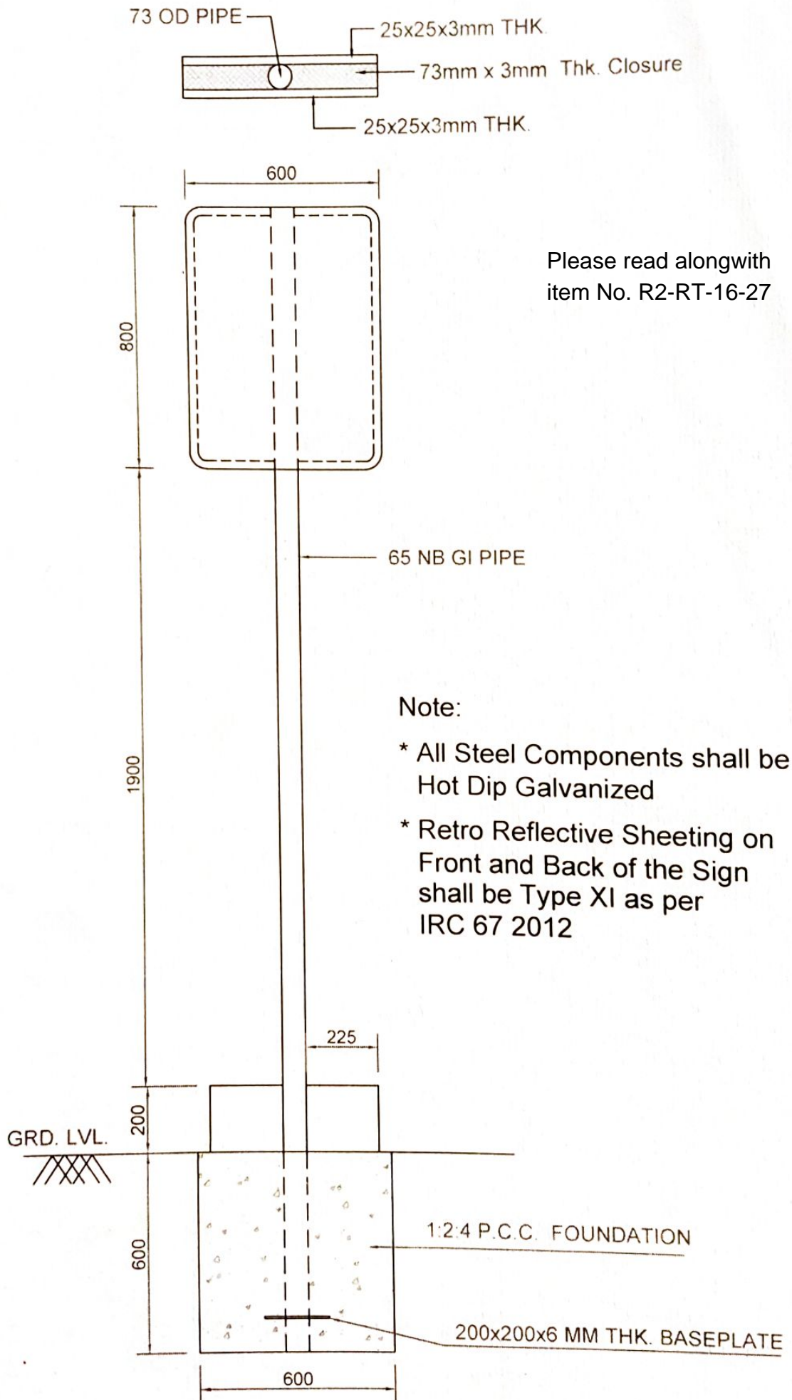
Facility Information Sign Drawing Refer Fig. F1
