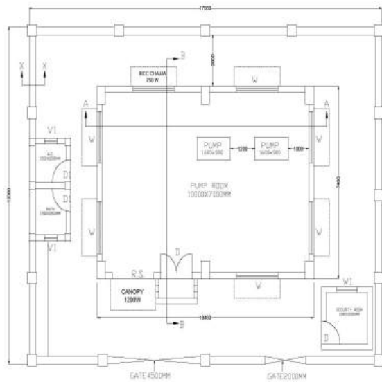
PLAN OF PUMP ROOM
