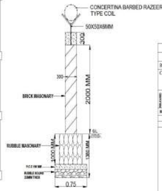
SECTION X-X
