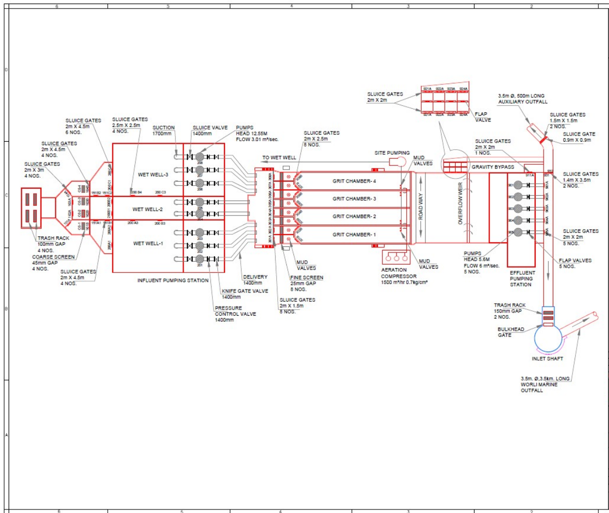
PROCESS FLOW DIAGRAM OF EXISTING WORLI WWTf
