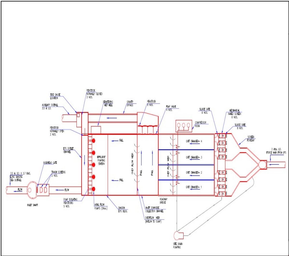
PROCESS FLOW DIAGRAM OF EXISTING BANDRA WWTf
