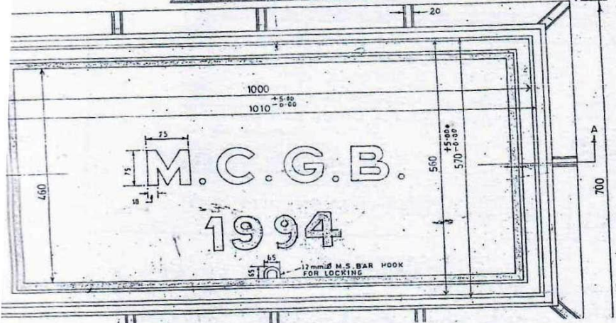
PLAN OF C.I. FRAME
