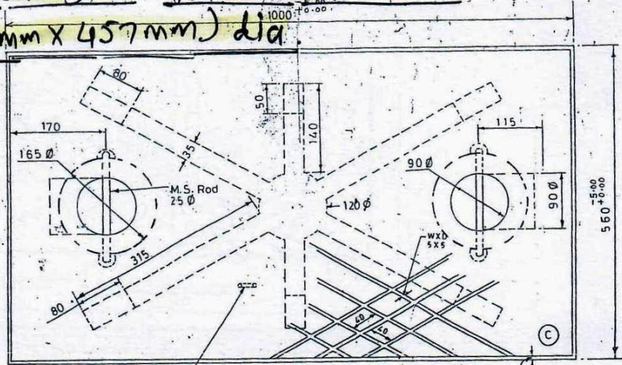
PLAN OF C.I. COVER
