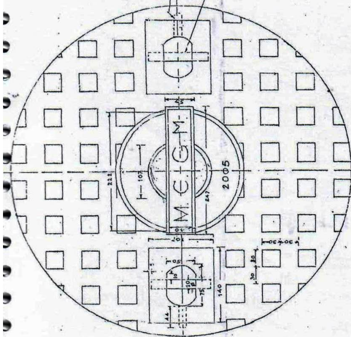
PLAN OF MANHOLE COVER (TOP)
