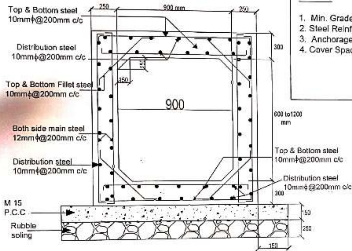
CASE 2 :- CLEAR WATER WAY WIDTH 900 MM
