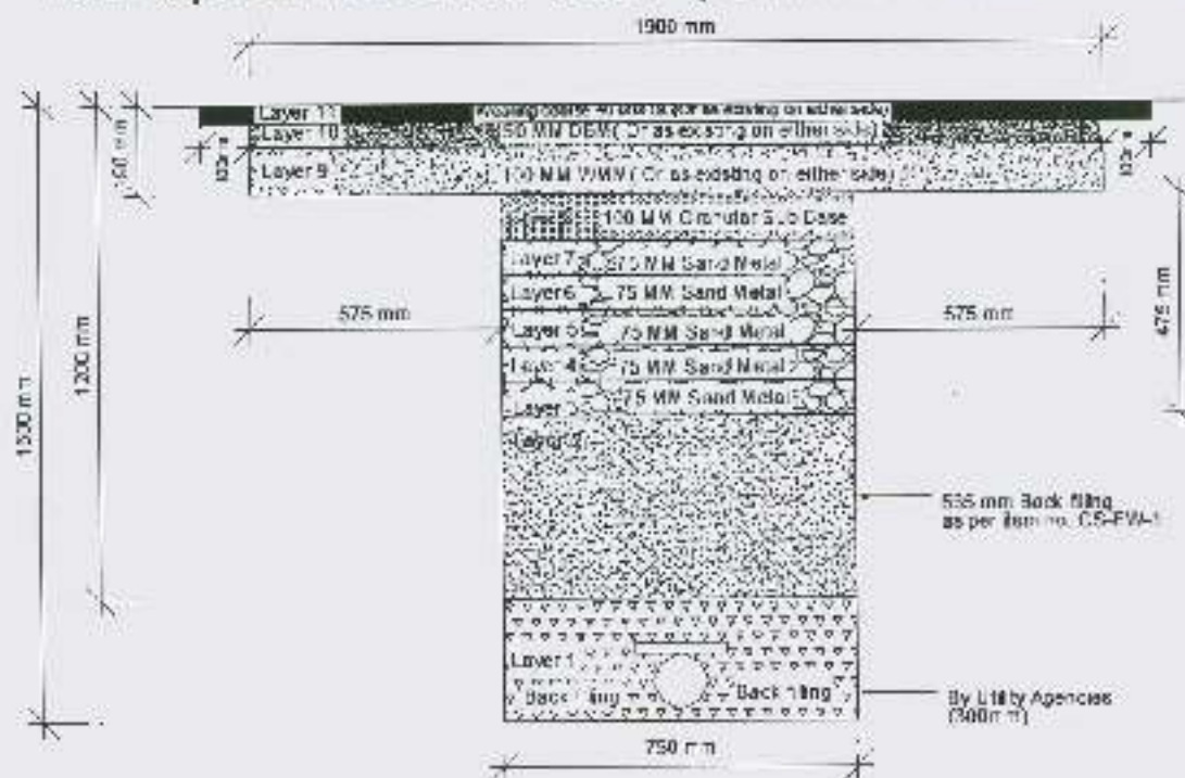
Layer wise details for item / materials to be used & its compaction.
