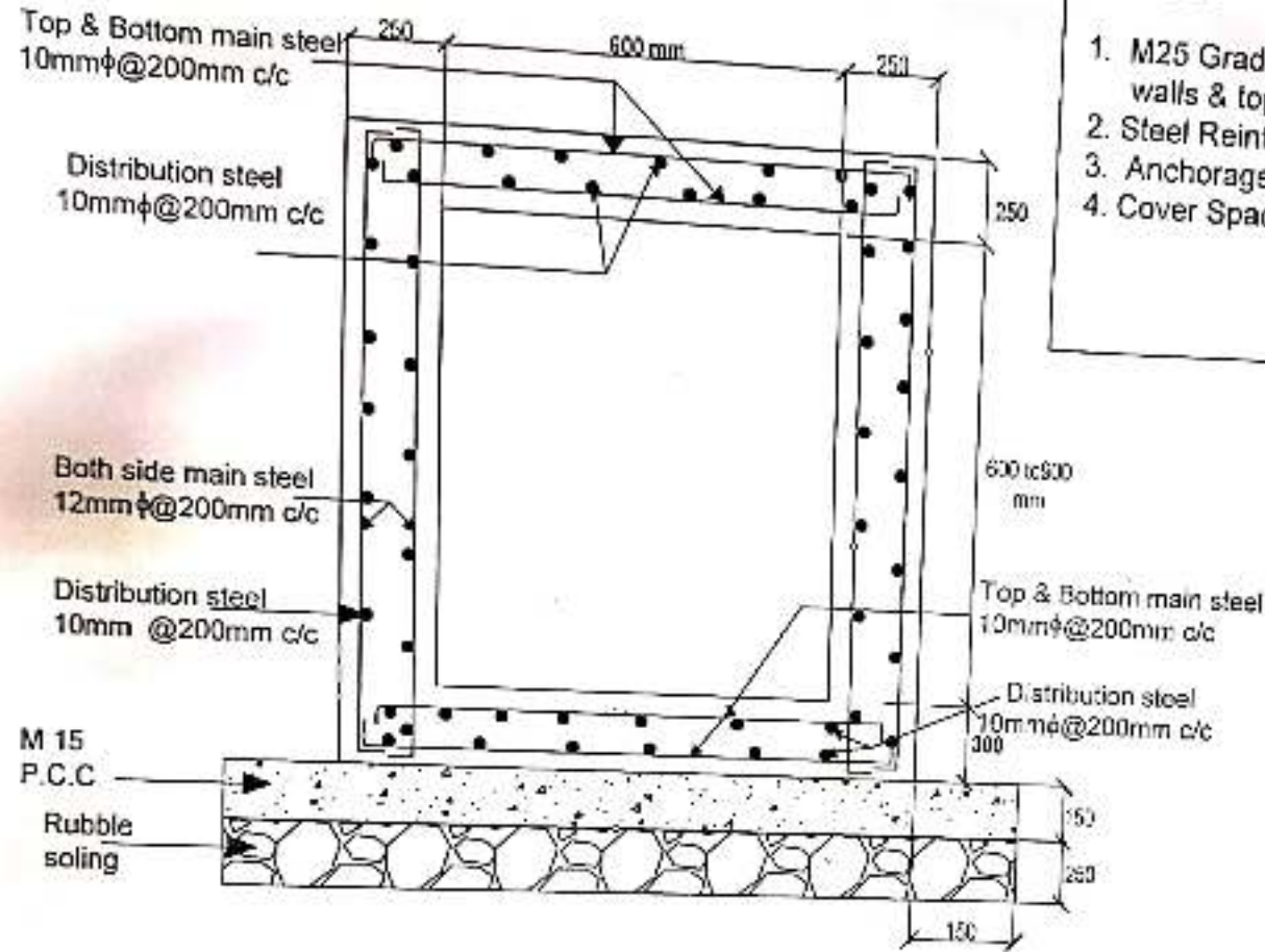
CASE 1 :- CLEAR WATER WAY WIDTH 600 MM
