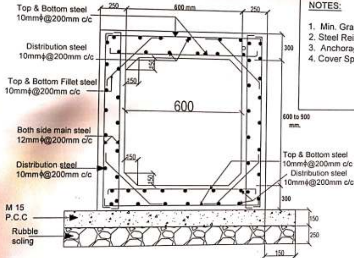
CASE 1 :- CLEAR WATER WAY WIDTH 600 MM
