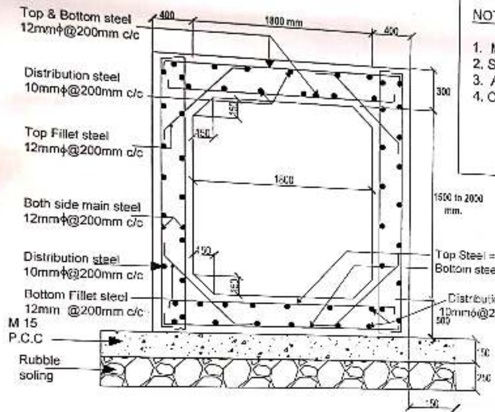
CASE 5:- CLEAR WATER WAY WIDTH 1800 MM
