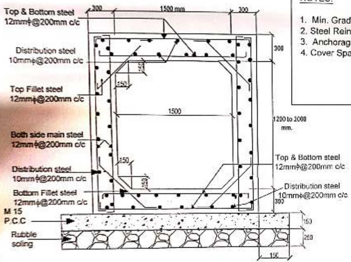
CASE 4 :- CLEAR WATER WAY WIDTH 1500 MM
