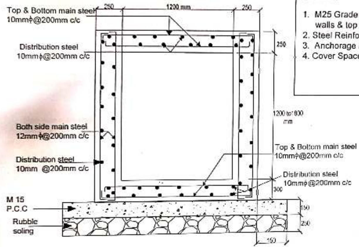
CASE 3 :- CLEAR WATER WAY WIDTH 1200 MM
