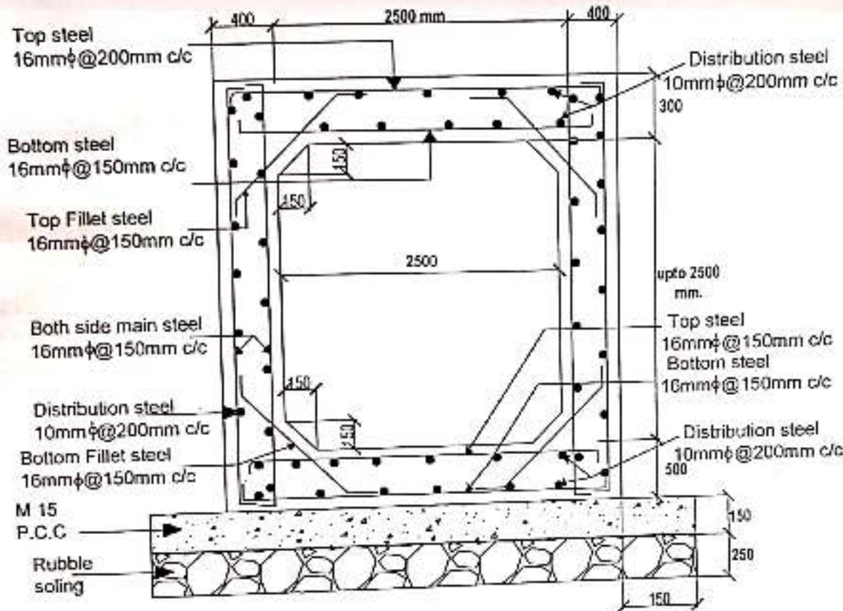
CASE 7 :- CLEAR WATER WAY WIDTH 2500 MM
