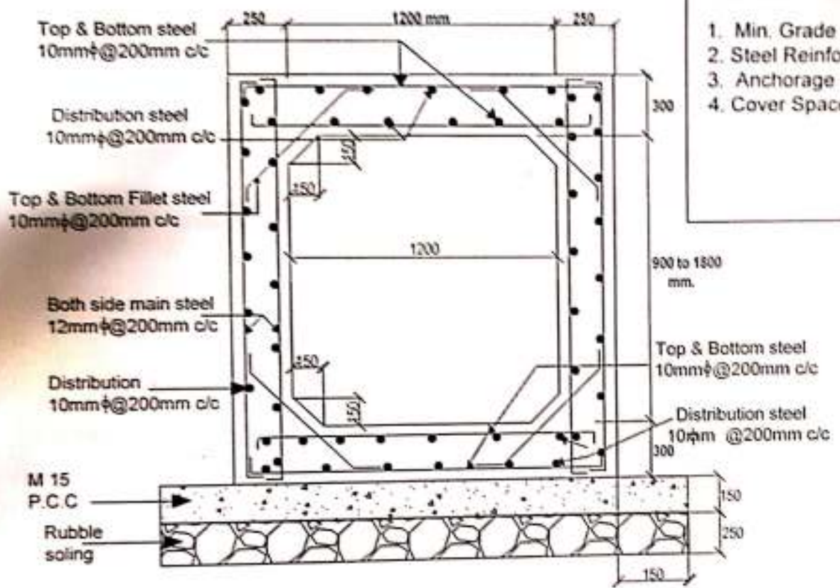
CASE 3 :- CLEAR WATER WAY WIDTH 1200 MM
