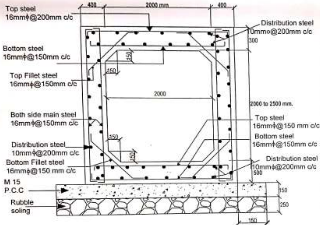
CASE 6 :- CLEAR WATER WAY WIDTH 2000 MM
