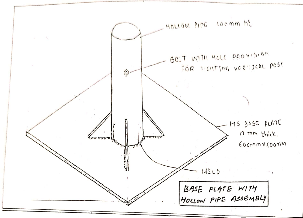
SKETCH 1 BASE PLATE WITH HOLLOW PIPE ASSEMBLY
