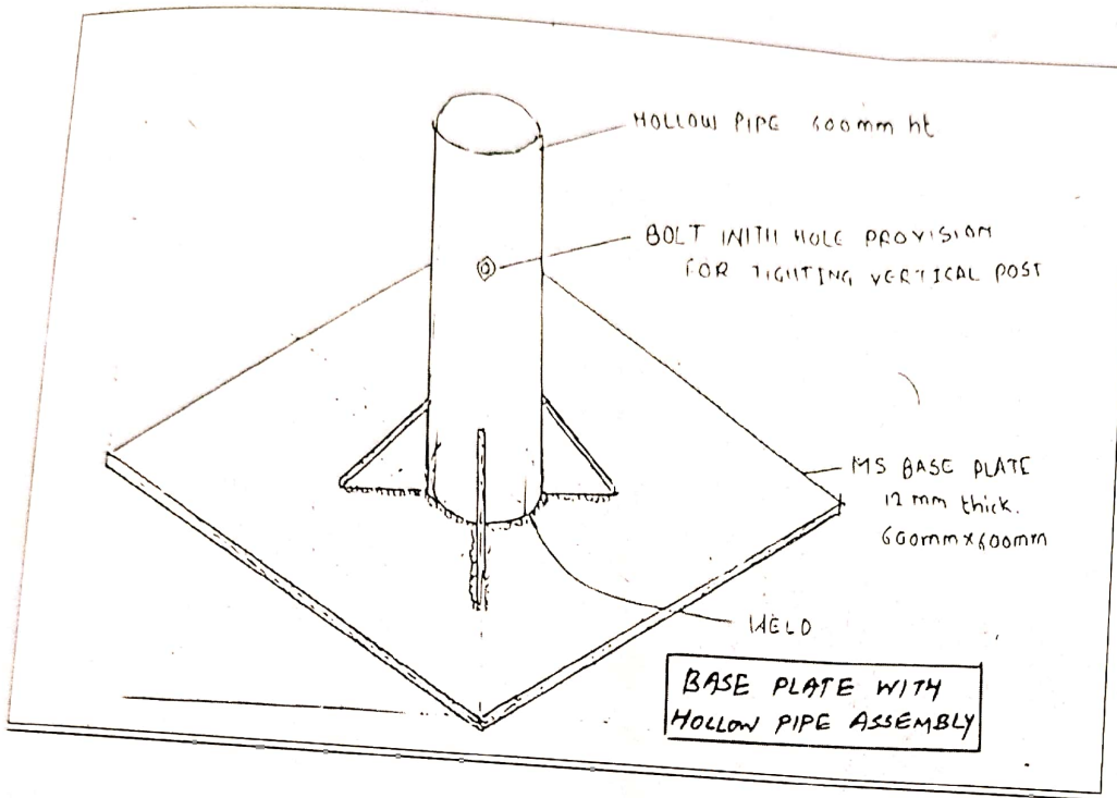
SKETCH 1 BASE PLATE WITH HOLLOW PIPE ASSEMBLY
